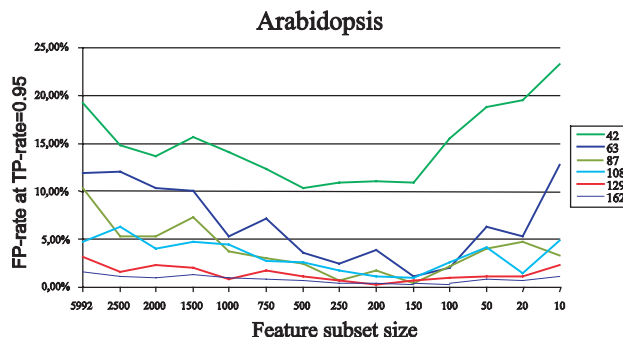
Fig. 3. Effect of feature selection on the classification performance for the new method FSS-SVM. The x -axis denotes the feature subset size, starting at the origin with the full feature set. Going further away from the origin, gradually more features are eliminated. The y -axis shows the classification performance.
